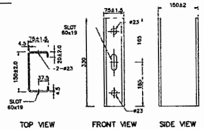
BLOCKOUT DETAILS SCALE 1 : 5
