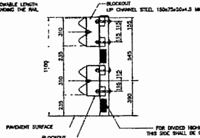
WHITE REFLECTIVE SHEETING TYPE I FOR DIVIDED HIGHWAY, THIS SIDE SHALL BE OMITTED
