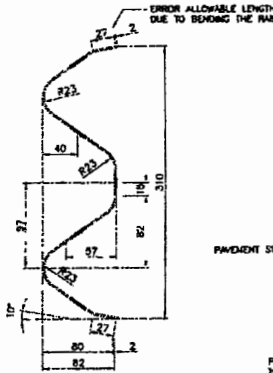
RAIL SECTION SCALE 1 : 3
