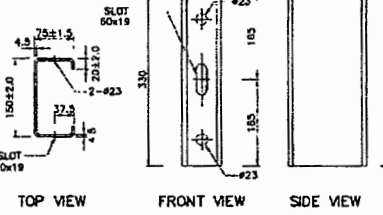
BLOCKOUT DETAILS SCALE 1 : 5
