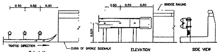
DETAIL "D" SCALE 1 : 25
