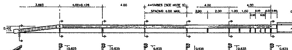
ELEVATION OF GUARDRAIL TO BRIDGE RAILING SCALE 1 : 75
