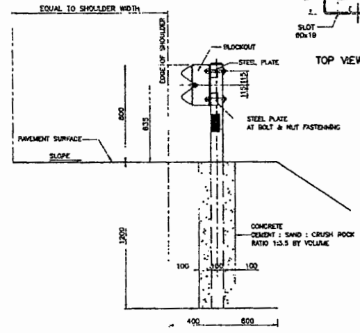
BLOCKOUT DETAILS SCALE 1 : 5
