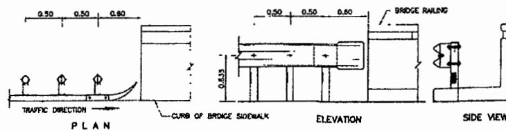
DETAIL "D" SCALE 1 : 25
