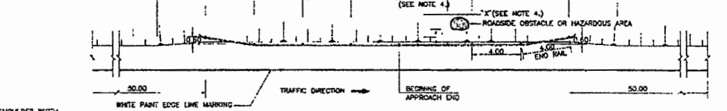
APPROACH END INSTALLATION FOR ROADSIDE OBSTACLE SCALE 1:150
