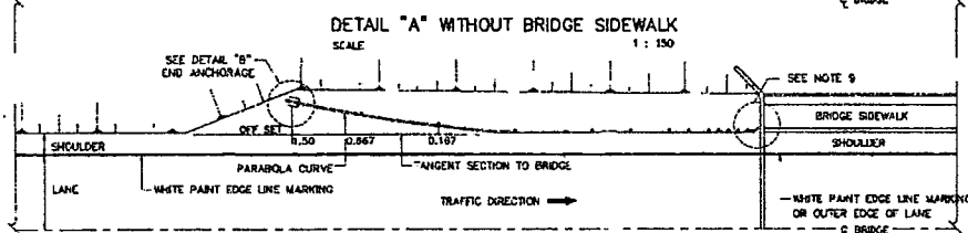
APPROACH END INSTALLATION FOR ROADSIDE OBSTACLE SCALE: 1:150
