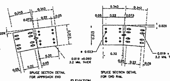
ELEVATION SCALE 1:50
