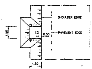
ON WALKWAY ON SHOULDER LOCATION OF LIGHTING POLE, AT GRADE NOT TO SCALE
