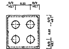
4 DUCT (2x2)
