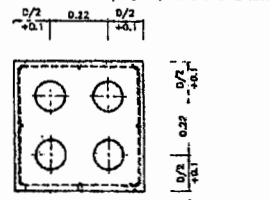
4 DUCT (2x2)
