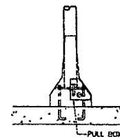
SECTION D-D NOT TO SCALE
