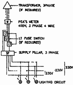
BLOCK DIAGRAM 2
