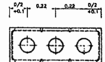
3 DUCT (3x1) TYPICAL DUCT BANK SECTION SCALE 1:10
