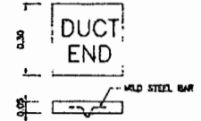
DUCT MARKER DETAIL SCALE 1:10
