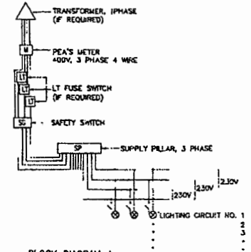
BLOCK DIAGRAM 4
