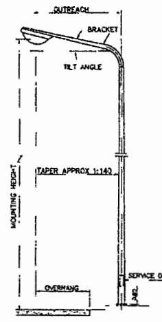
LIGHTING POLE, SINGLE ARM NOT TO SCALE
