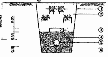
TYPICAL DETAIL: DIRECT BURIAL SCALE NONE
