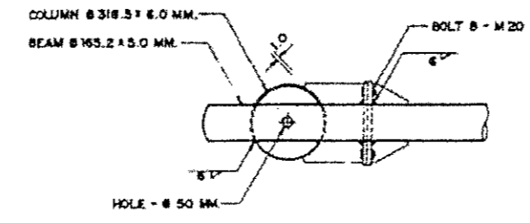
TOP OF STEEL POLE AND JOINT DETAIL SCALE 1:15
