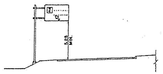
SECTION FOR OVERHANGING TRAFFIC SIGN NOT TO SCALE
