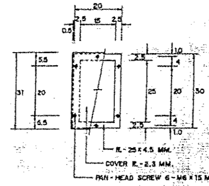
SECTION C-C SCALE 1:17.5
