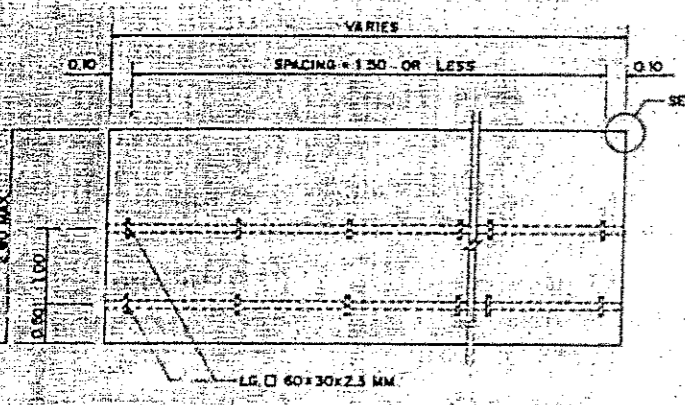
ERECTION FOR SIGN BOARD SCALE 1:50
