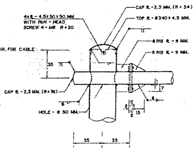
DETAIL 1 SCALE 1:15
