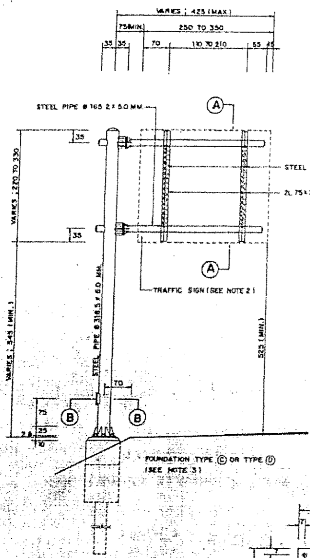
STEEL POLE FOR OVERHANG TRAFFIC SIGN TYPE 3 AT SIDE SLOPE SCALE 1:150
