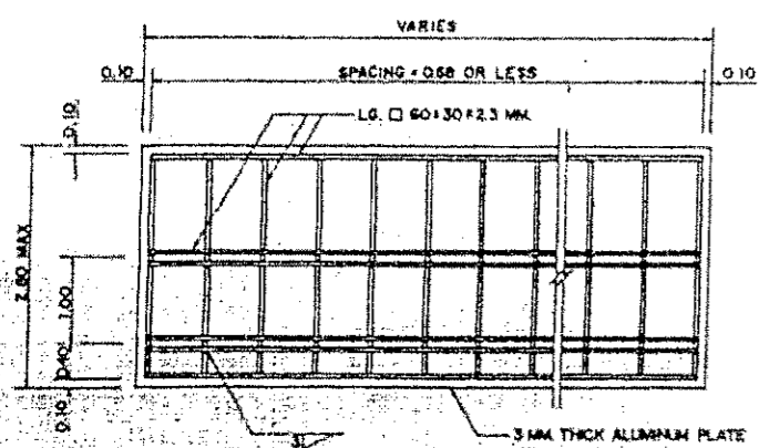
TYPICAL SIGN FRAME SCALE 1:50
