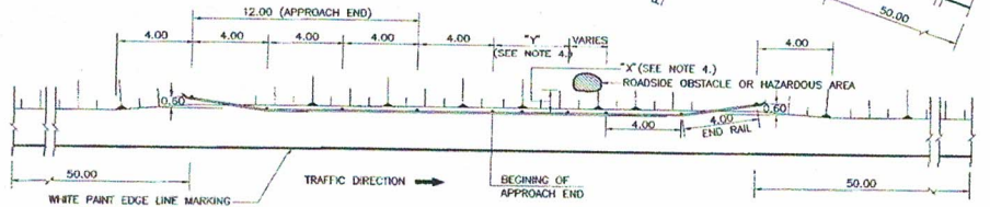
APPROACH END INSTALLATION FOR ROADSIDE OBSTACLE SCALE 1:150
