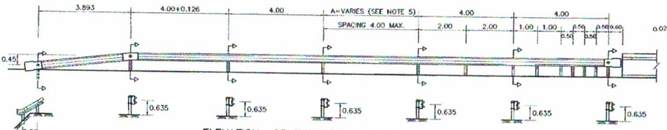
ELEVATION OF GUARDRAIL TO BRIDGE RAILING SCALE 1:75
