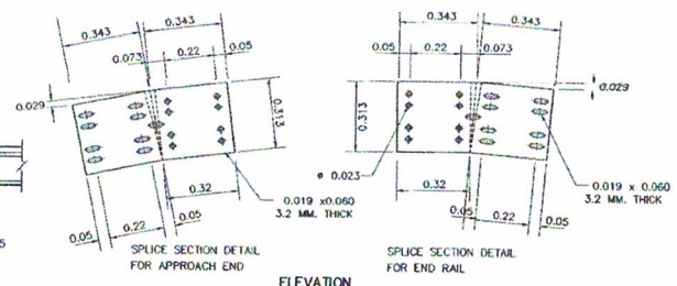
SPLICE SECTION NOT TO SCALE
