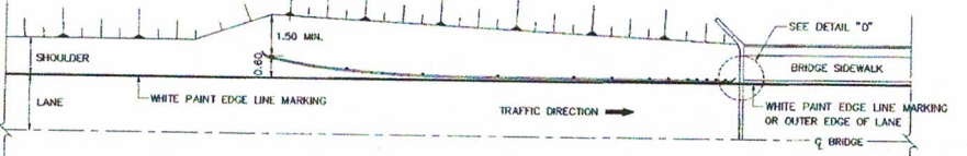
INSTALLATION OF W-BEAM GUARDRAIL AT BRIDGE APPROACH WITH BRIDGE SIDEWALK (ROADWAY SHOULDER WIDER THAN BRIDGE) SCALE 1:150
