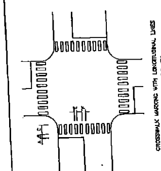
CROSSWALK MARKINGS WITH LONGITUDINAL LINES FOR IMPROVED VISIBILITY
