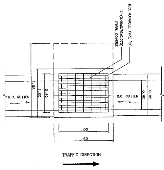
PLAN OF R.C. GUTTER AND R.C. MANHOLE TYPE 'C' NOT TO SCALE
