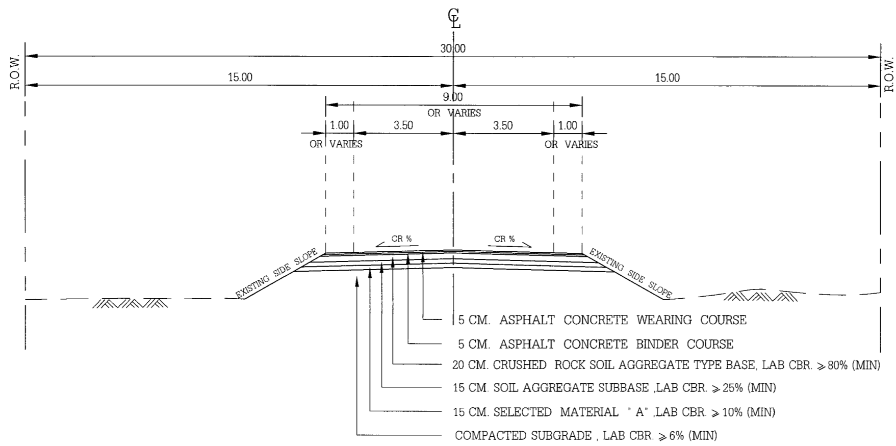
EXISTING CROSS SECTION STA.69+000 - STA.69+316 STA.69+366 - STA.72+920
