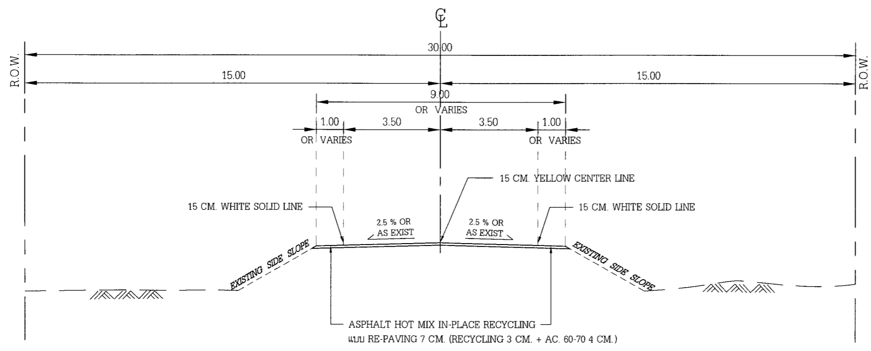
TYPICAL CROSS SECTION STA.69+000 - STA.69+316 STA.69+366 - STA.72+920
