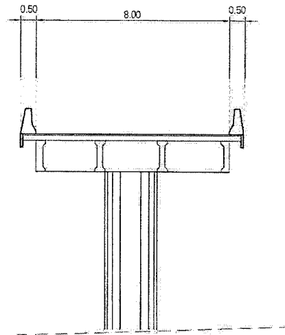
EXISTING CROSS SECTION STA.37+488
