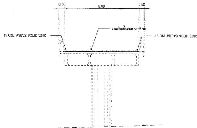
TYPICAL CROSS SECTION STA.37+488
