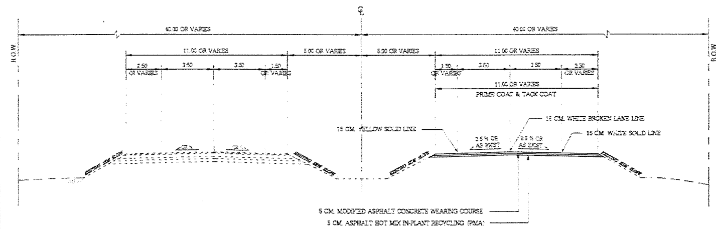
TYPICAL CROSS SECTION STA.106-700 - STA.107-765 (RT)
