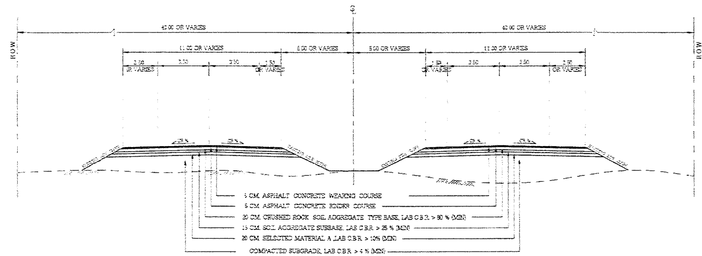
EXISTING CROSS SECTION STA.106+700 - STA.107+765 (RT)
