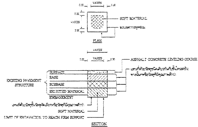
SOFT MATERIAL EXCAVATION AND REPLACEMENT
