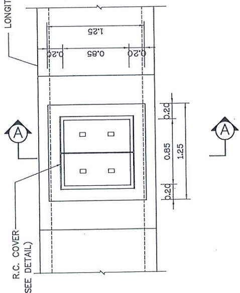
PLAN INLET SHAFT OVER R.C. BOX CULVERT NOT TO SCALE
