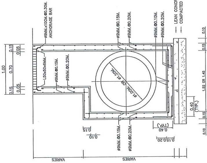
SECTION A - A FOR REINFORCEMENT NOT TO SCALE
