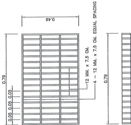
DETAIL FOR STEEL COVER NOT TO SCALE
