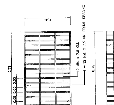
DETAIL FOR STEEL COVER
