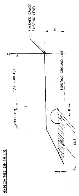
GENERAL RECOMMENDATION FOR FILL OR CUT SLOPE CONSTRUCTION
