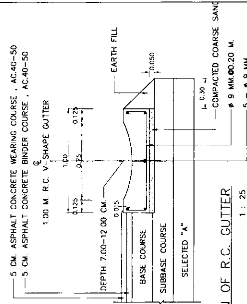
SECTION OF R.C. GUTTER SCALE 1 : 25
