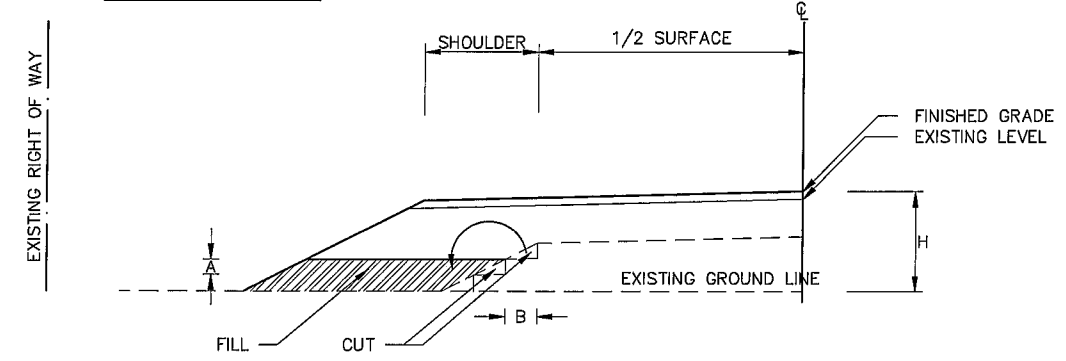
GENERAL RECOMMENDATION FOR FILL OR CUT SLOPE CONSTRUCTION
