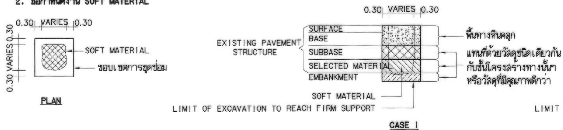
DETAIL OF SOFT SPOT EXCAVATION AND MAINTAINANCE
