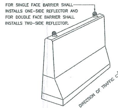
INSTALLATION REFLECTIVE TARGET ON BARRIER
