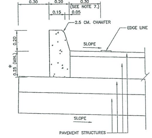
CONCRETE CURB NOT TO SCALE
