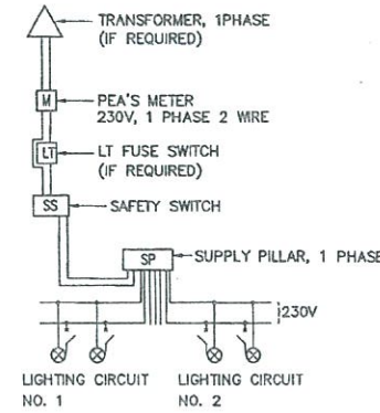
BLOCK DIAGRAM 3
