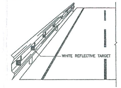
INSTALLATION REFLECTIVE TARGET ON GUARDRAIL
