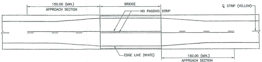
MARKING AT BRIDGE APPROACH
