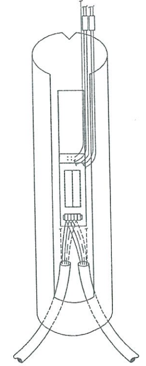
TYPE 2: FOR LIGHTING POLE, DOUBLE ARM(2 PHASE)
