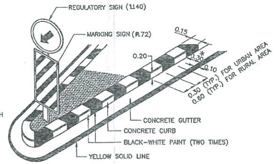
PAINT MARKING ON CONCRETE CURB
