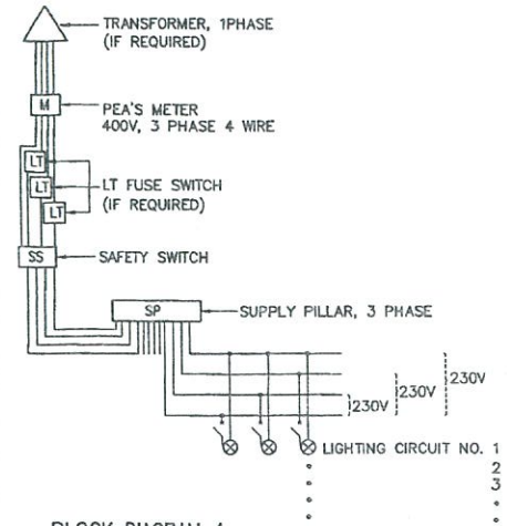
BLOCK DIAGRAM 4
