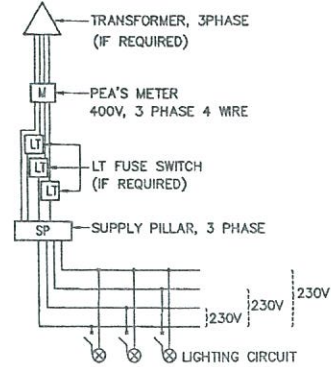
BLOCK DIAGRAM 2
