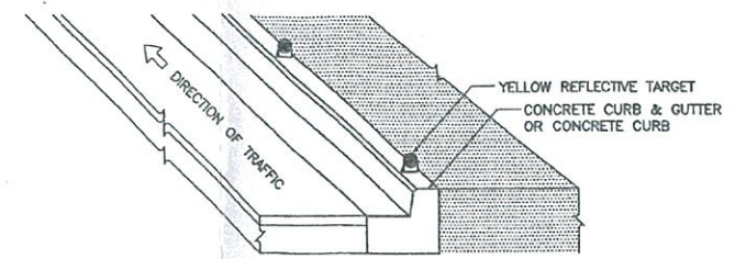
INSTALLATION REFLECTIVE TARGET ON CURB MEDIAN
