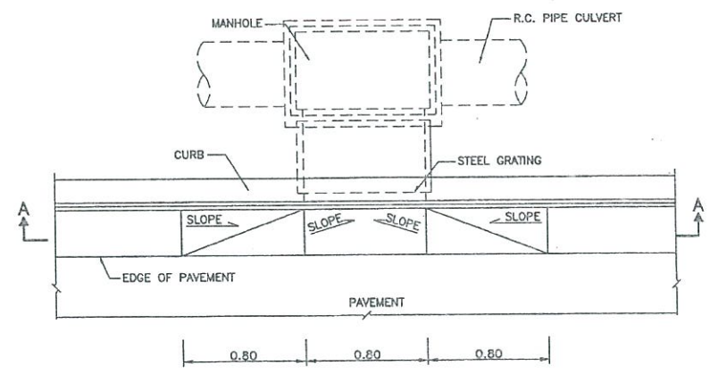
PLAN OF INLET DRAIN NOT TO SCALE
