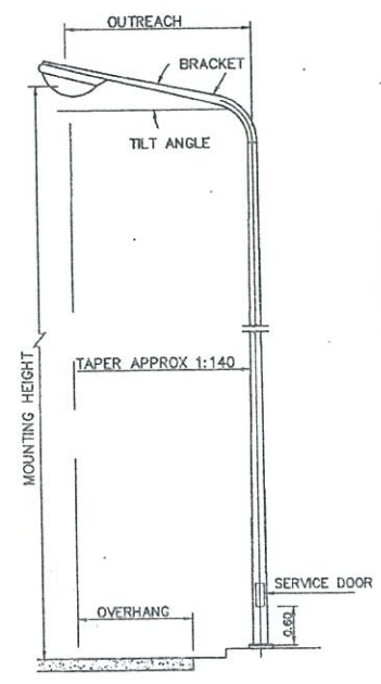
LIGHTING POLE, SINGLE ARM NOT TO SCALE
