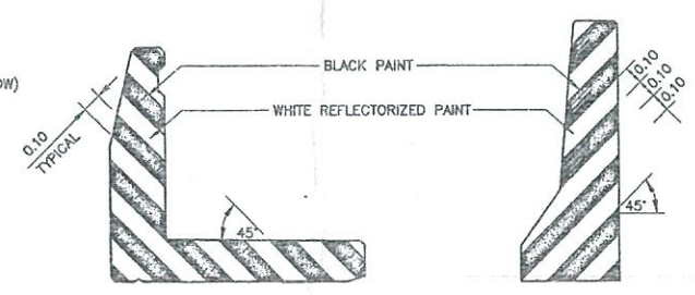
MARKING AT ENDS OF BRIDGE BARRIER
