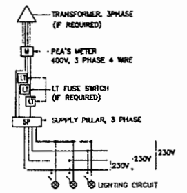
BLOCK DIAGRAM 2
