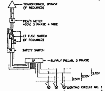
BLOCK DIAGRAM 4
