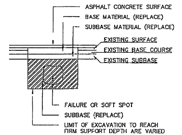
(OVERLAY SECTION)
