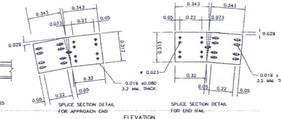
SPlice SECTION NOT TO SCALE
