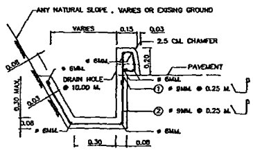
TYPE V CONCRETE DITCH AT HILLSIDE SCALE 1:12.5
