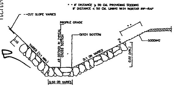
TYPE III MORTAR RIP-RAP DITCH LINING SCALE 1:10
