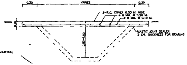
DETAIL FOR R.C. COVER FOR CROSS WALK SCALE 1:10
