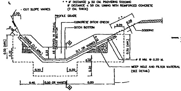
TYPE II REINFORCED CONCRETE DITCH LINING SCALE 1:10
