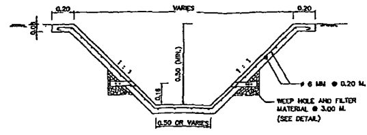
TYPE IV SIDE DITCH FOR VILLAGE SECTION SCALE 1:10
