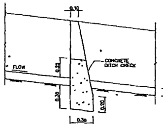
SECTION A-A DETAIL FOR DITCH CHECK SCALE 1:10
