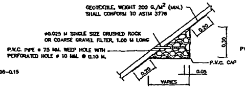
DETAIL OF WEEP HOLE AND FILTER MATERIAL SCALE 1:10
