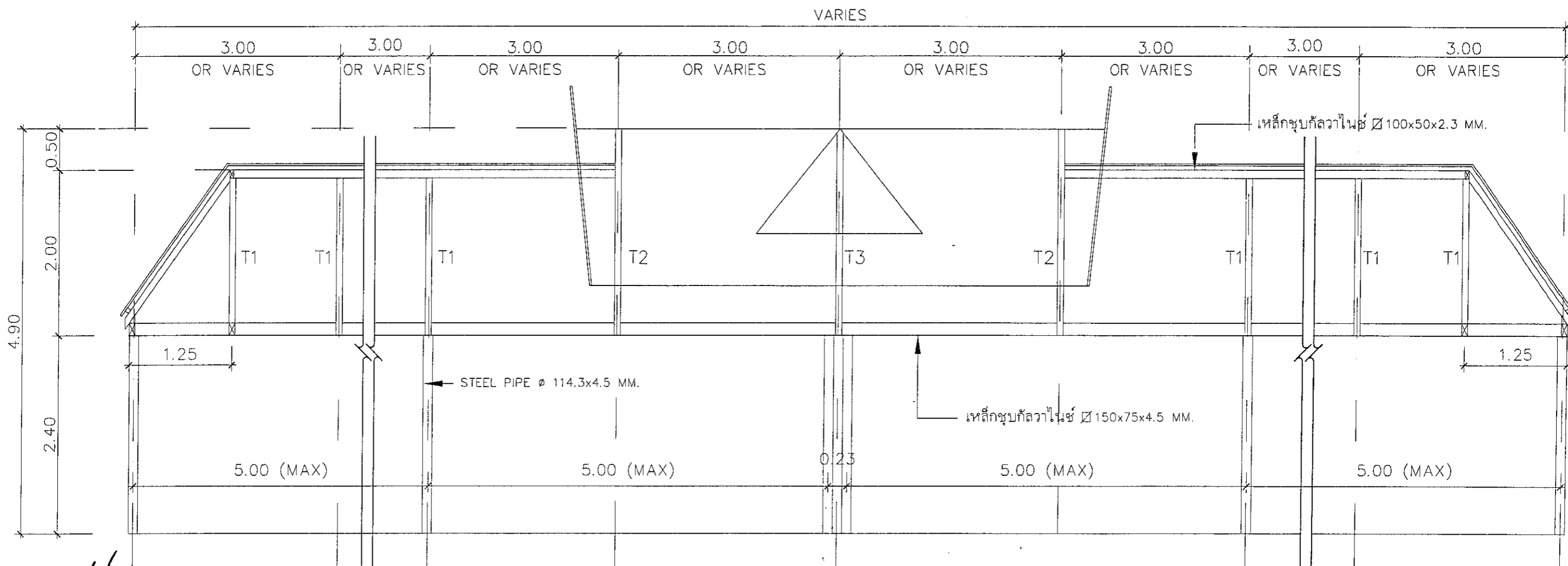
SECTION B - B
