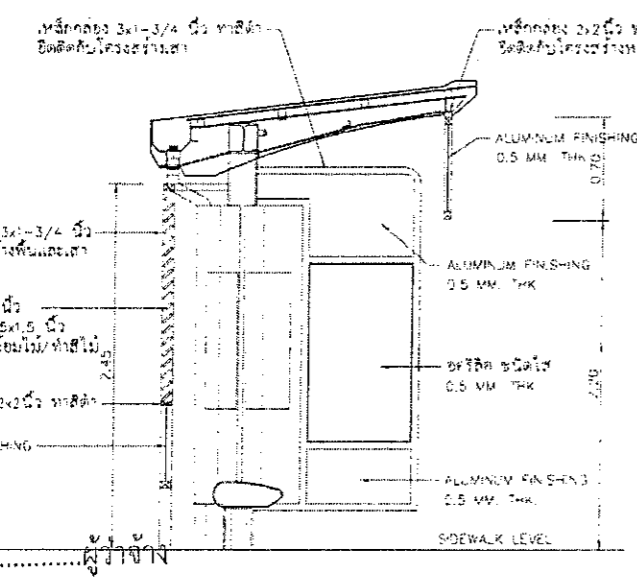
SECTION A SCALE 1:50
