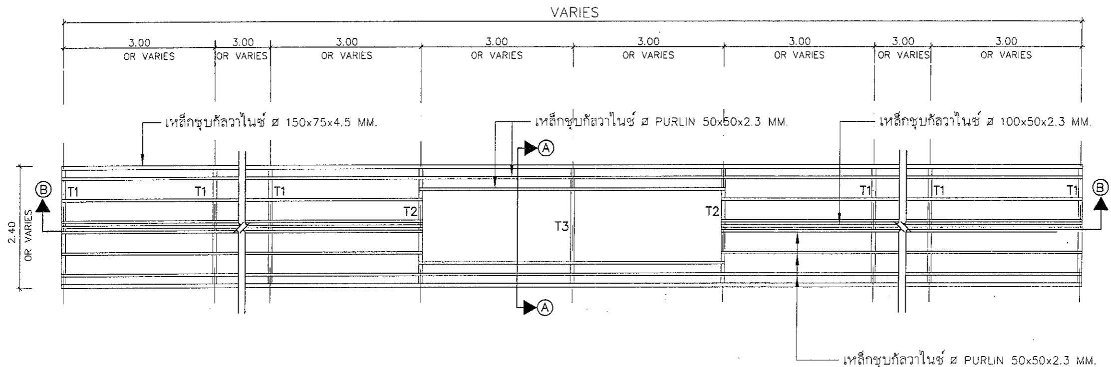
LOWER ROOF FRAMING PLAN SCALE 1:75
