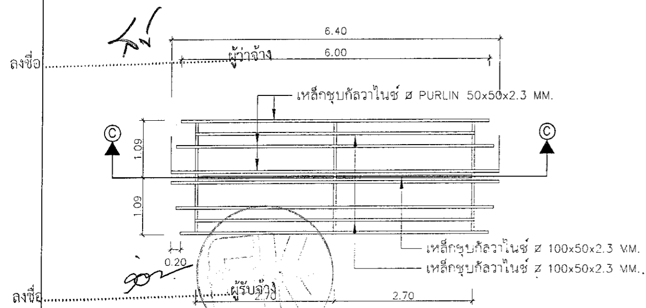
UPPER ROOF FRAMING PLAN SCALE 1:75
