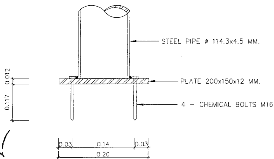
STEEL PLATE DETAILS
