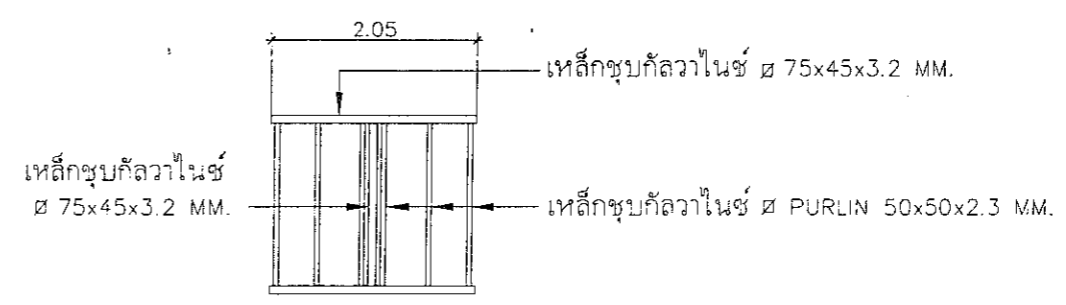
TOP ROOF FRAMING PLAN SCALE 1:75
