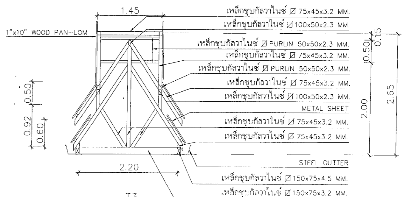
T3 SCALE 1:50
