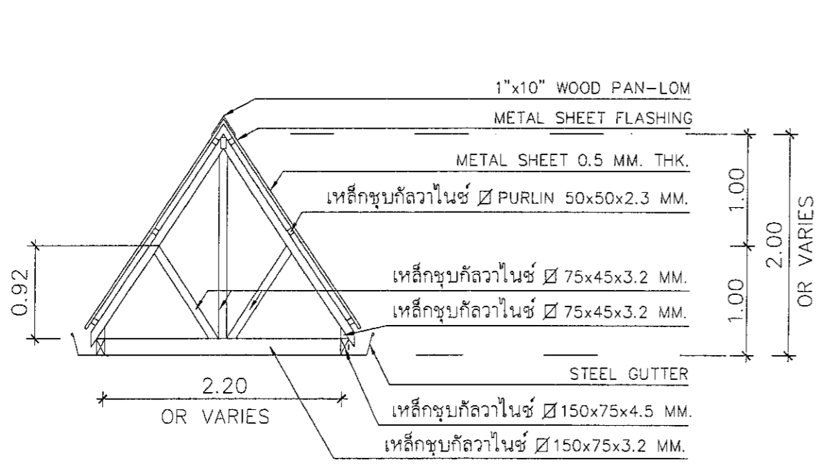
T1 SCALE 1:50
