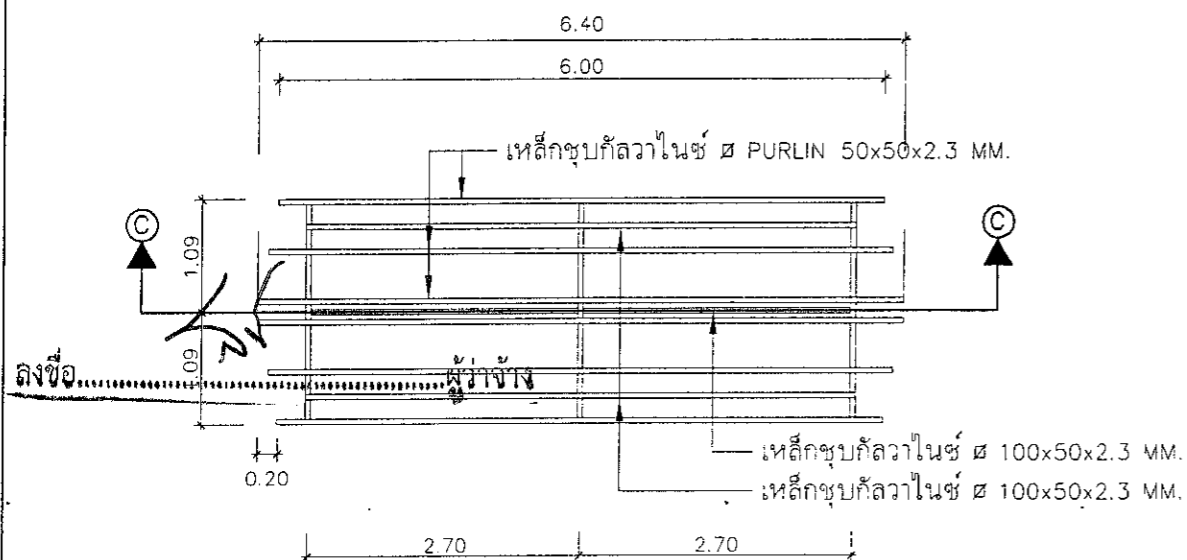
UPPER ROOF FRAMING PLAN
