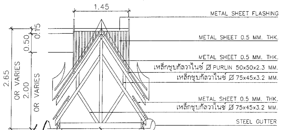
T1 SCALE 1:50
