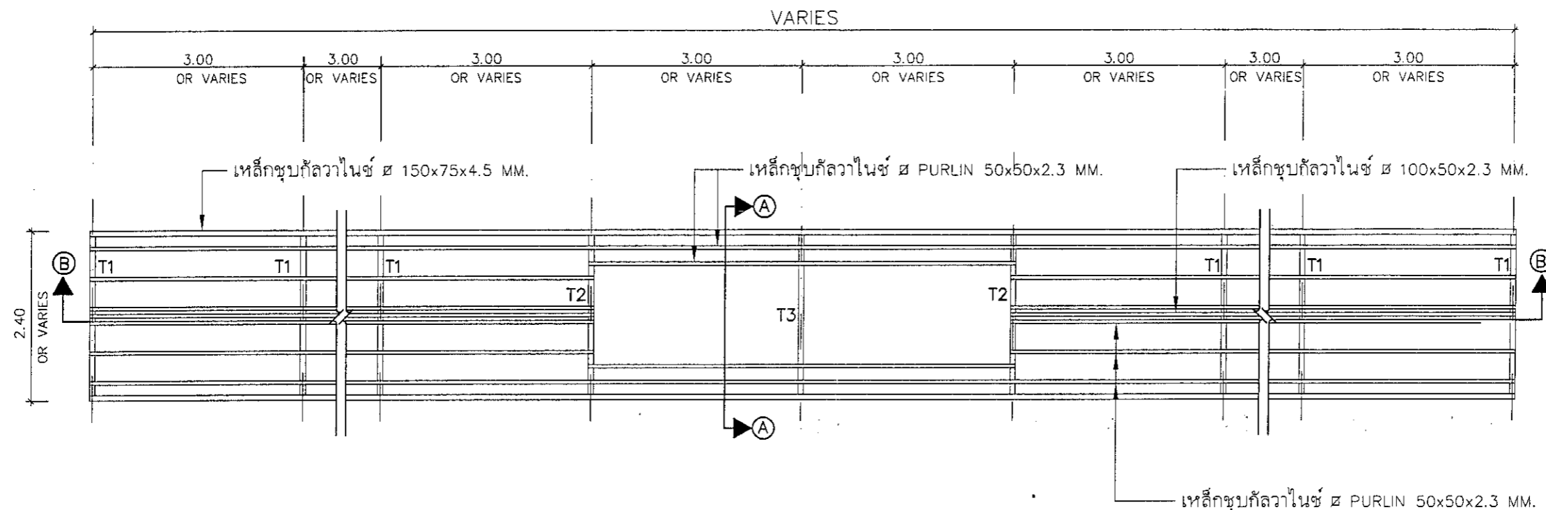
LOWER ROOF FRAMING PLAN
