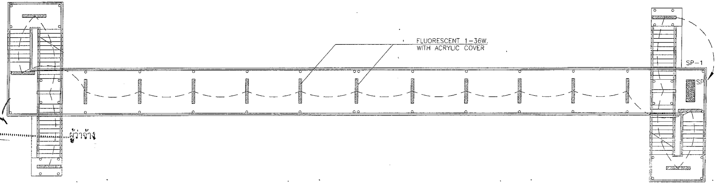
LIGHTING PLAN FOR PEDESTRIAN WITH ROOF SCALE NOT TO SCALE
