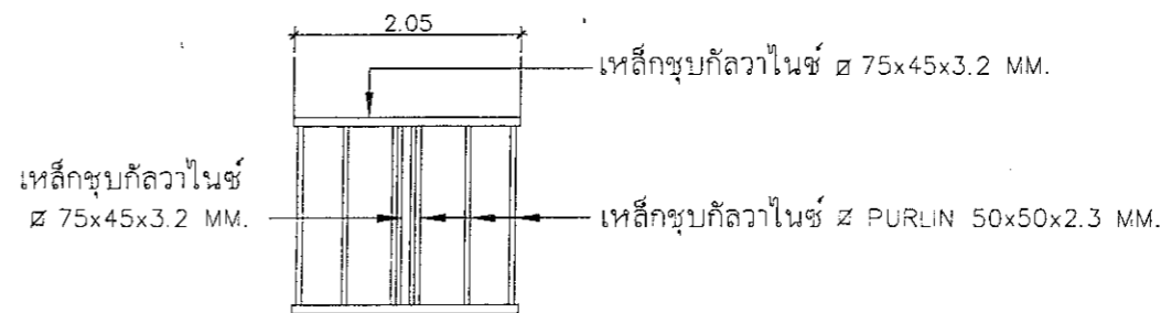
TOP ROOF FRAMING PLAN
