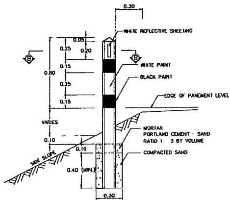
DETAIL "1" SCALE 1 : 15
