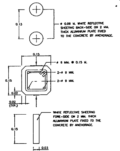
SECTION B - B CONCRETE TYPE SCALE 1 : 4
