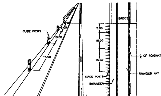
GUIDE POST INSTALLATION AT BRIDGE APPROACH NOT TO SCALE
