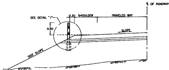
SECTION A - A CONCRETE TYPE NOT TO SCALE
