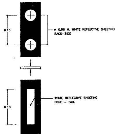
DETAIL "2" SCALE 1 : 4
