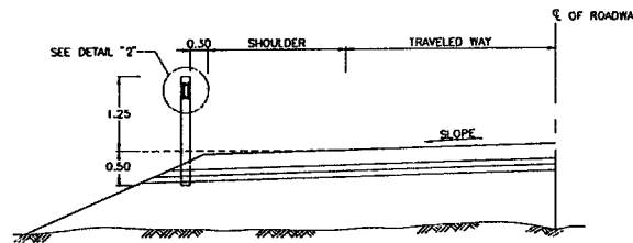
GUIDE POST INSTALLATION AT BRIDGE APPROACH NOT TO SCALE
