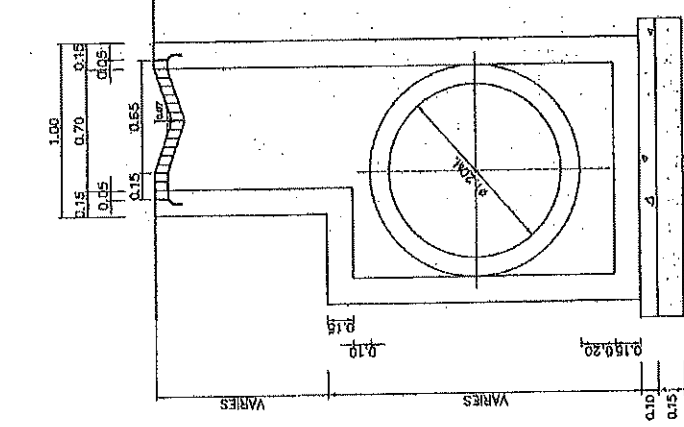
SECTION (A)-(A) FOR REINFORCEMENT
