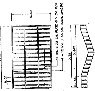
DETAIL FOR SPECIAL STEEL COVER NOT TO SCALE
