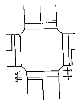
LANE LINE MARKINGS NET SCALE
