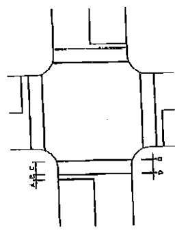
CROSSWALK MARKING WITH LONGITUDINAL LINES FOR ADDED VISIBILITY SCALE NOT
