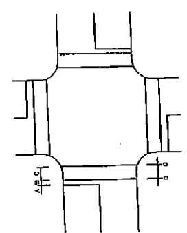
STANDARD CROSSWALK MARKING CROSSWALK MARKINGS NOT TO SCALE
