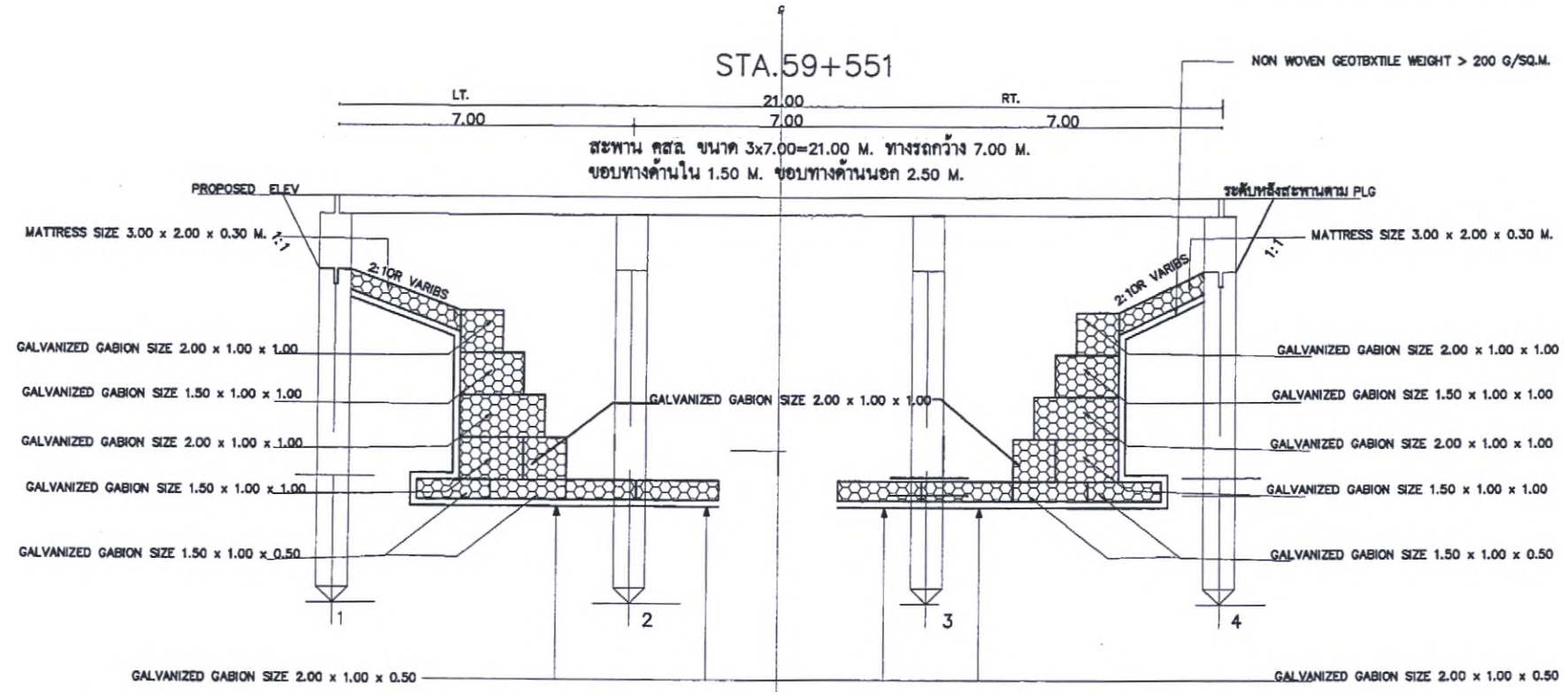
TYPICAL CROSS - SECTION A - A SCALE NO SCALE
