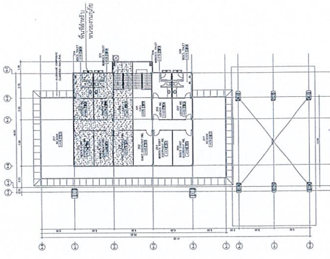
PLAN FLOOR 2 SCALE 1:200
