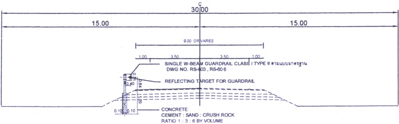
TYPICAL CROSS - SECTION A - A SCALE : NO SCALE
