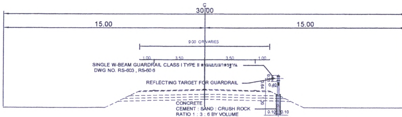
TYPICAL CROSS - SECTION B - B SCALE : NO SCALE
