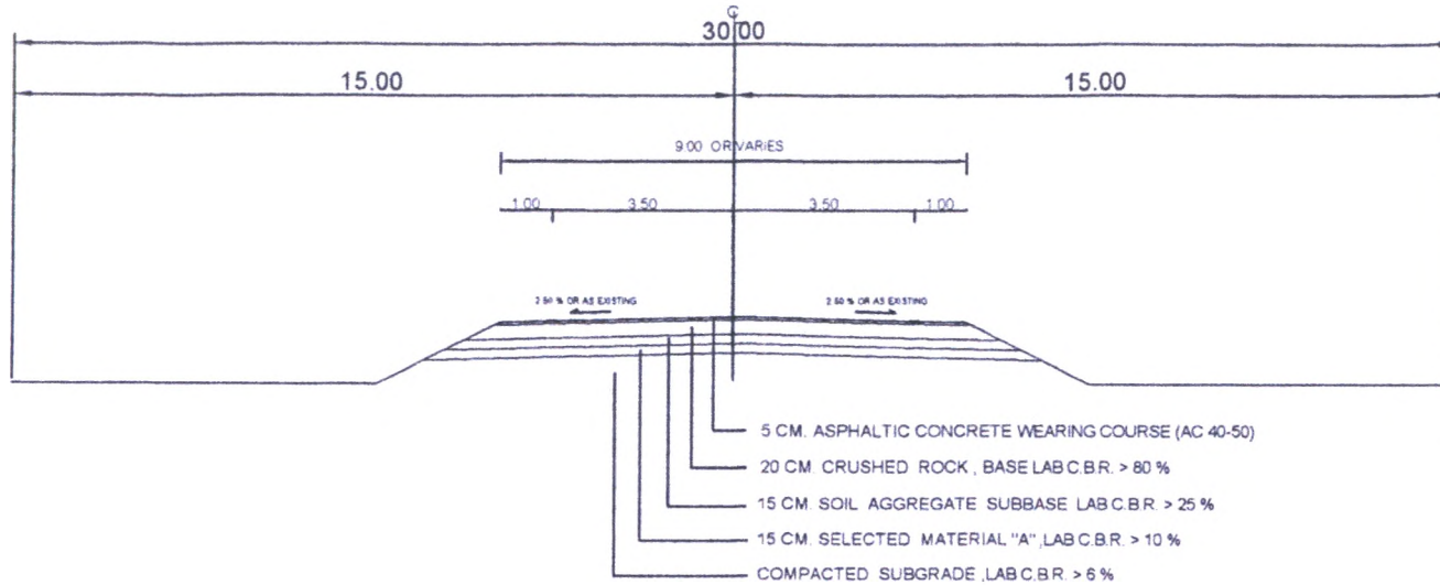
TYPICAL CROSS - SECTION B - B SCALE : NO SCALE
