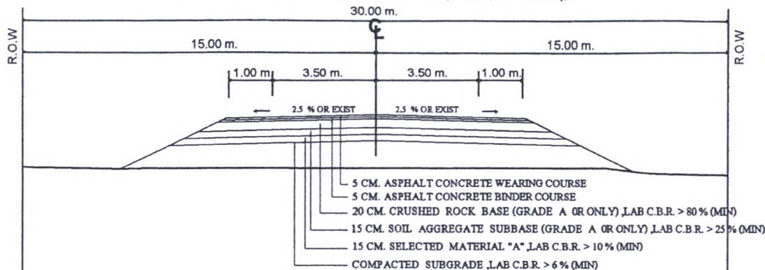
TYPICAL CROSS - SECTION B - B
