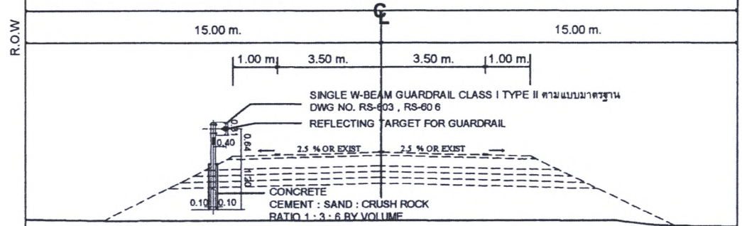
TYPICAL CROSS - SECTION A - A
