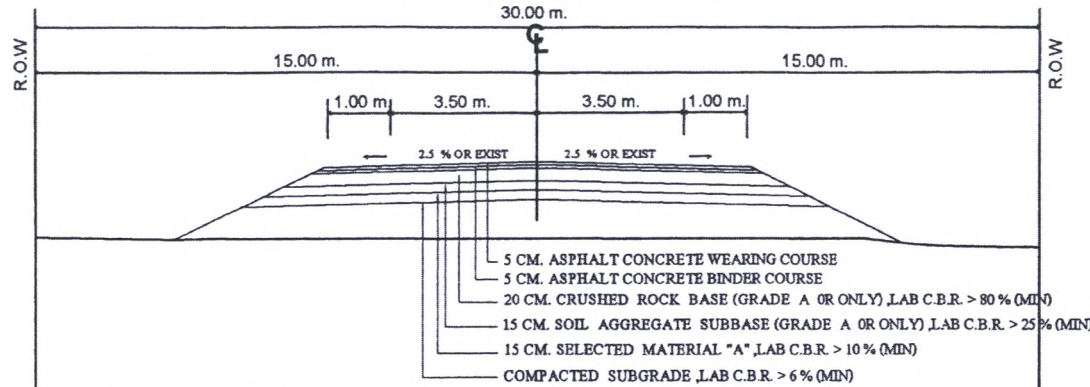
TYPICAL CROSS - SECTION A - A
