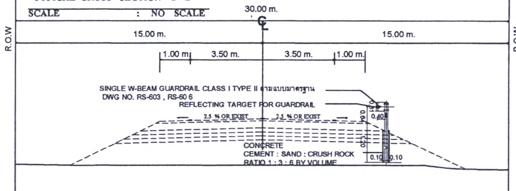
TYPICAL CROSS - SECTION B - B
