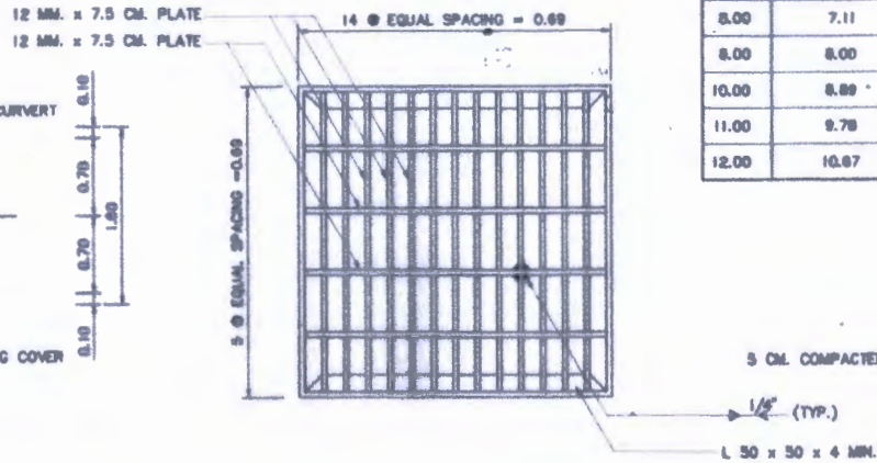
STEEL GRATING COVER DETAILS SCALE 1:25
