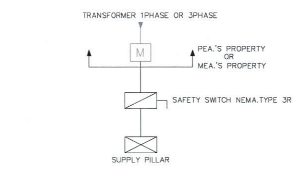
SINGLE LINE DIAGRAM FOR SUPPLY PILLAR
