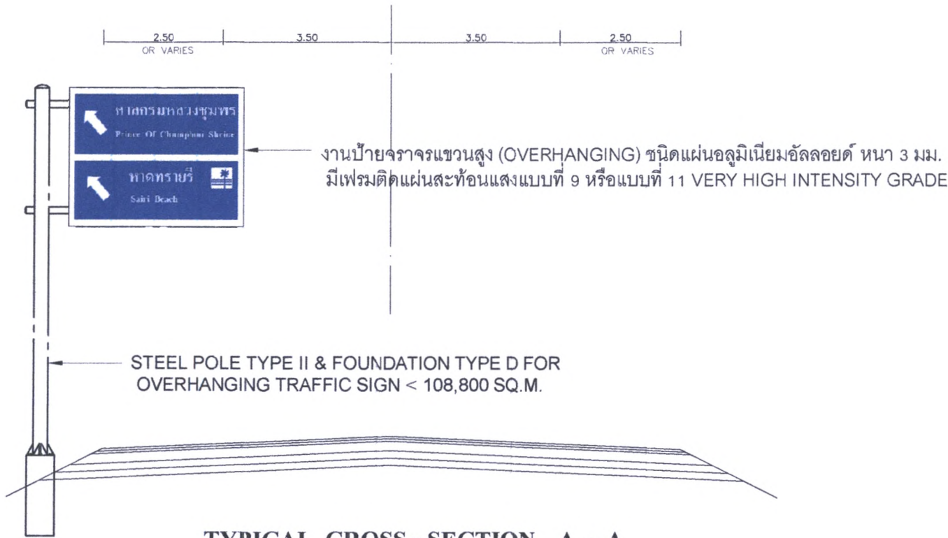
TYPICAL CROSS - SECTION A - A SCALE : NO SCALE
