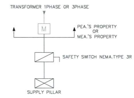
SINGLE LINE DIAGRAM FOR SUPPLY PILLAR
