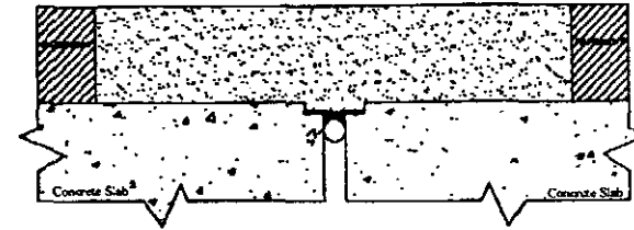
Joint Detail ②
