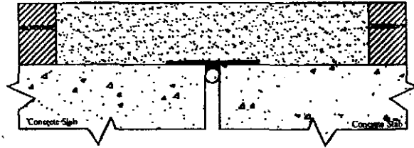
Joint Detail ①
