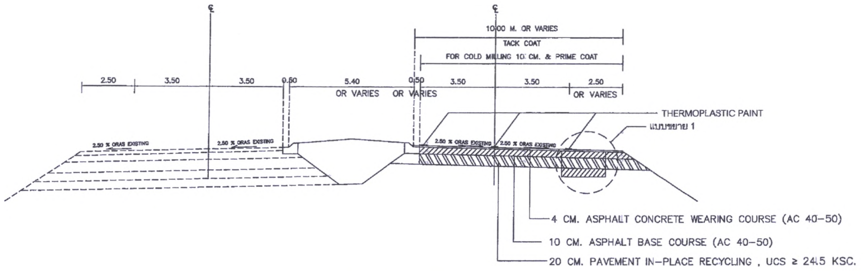
TYPICAL CROSS SECTION STA. 486+268 - STA. 487+903 RT.
