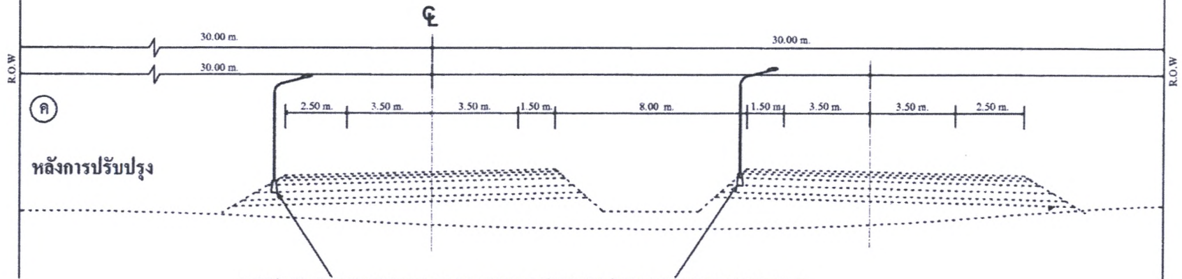
TYPICAL CROSS - SECTION C - C SCALE : NO SCALE
