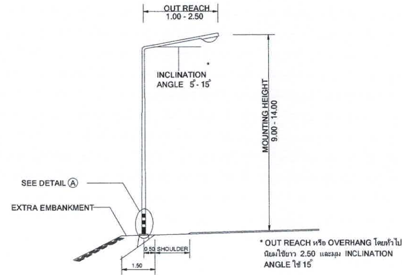
SINGLE BRACKET LIGHTING POLE
