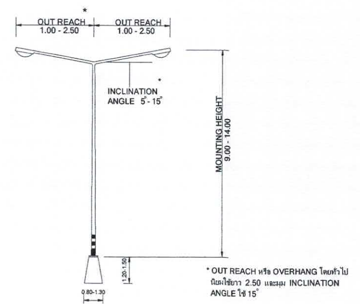
DOUBLE BRACKET LIGHTING POLE
