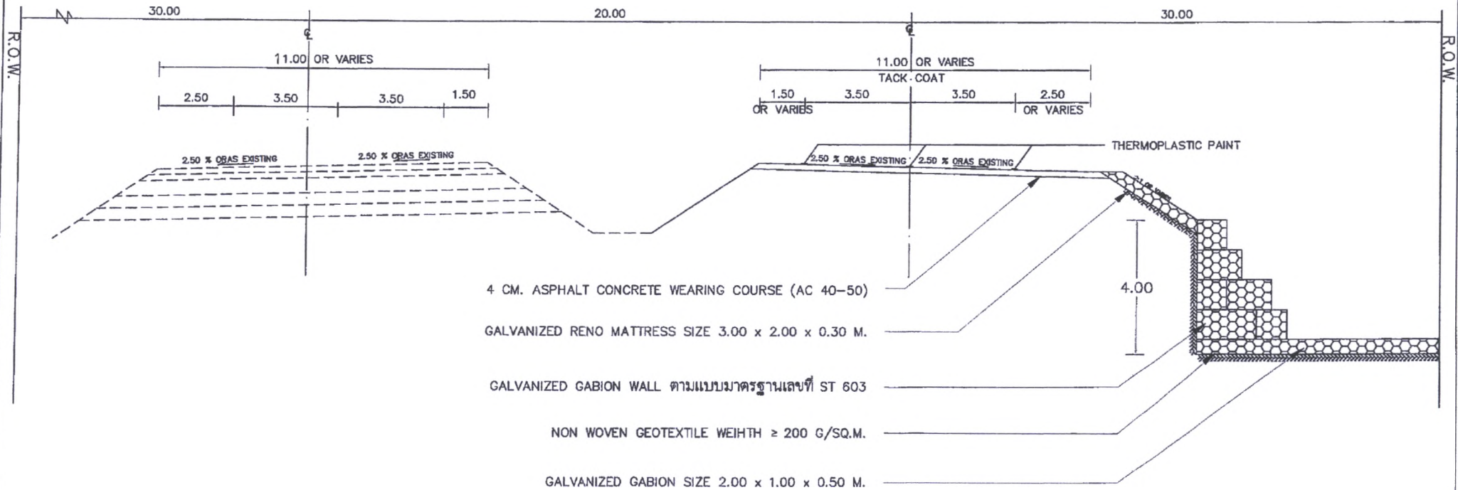
TYPICAL CROSS SECTION C-C
