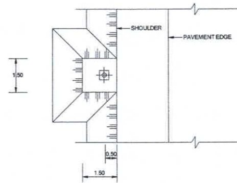
LOCATION OF LIGHTING POLE
