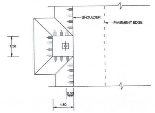
LOCATION OF LIGHTING POLE
