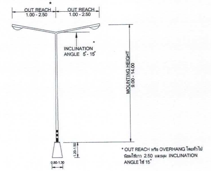
DOUBLE BRACKET LIGHTING POLE
