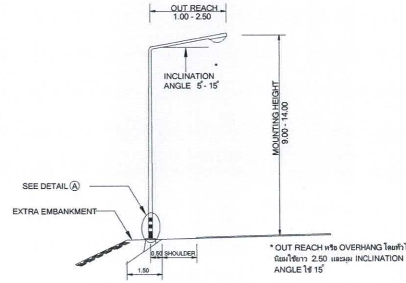
SINGLE BRACKET LIGHTING POLE
