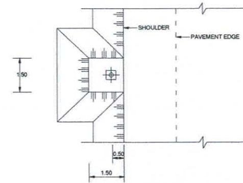
LOCATION OF LIGHTING POLE
