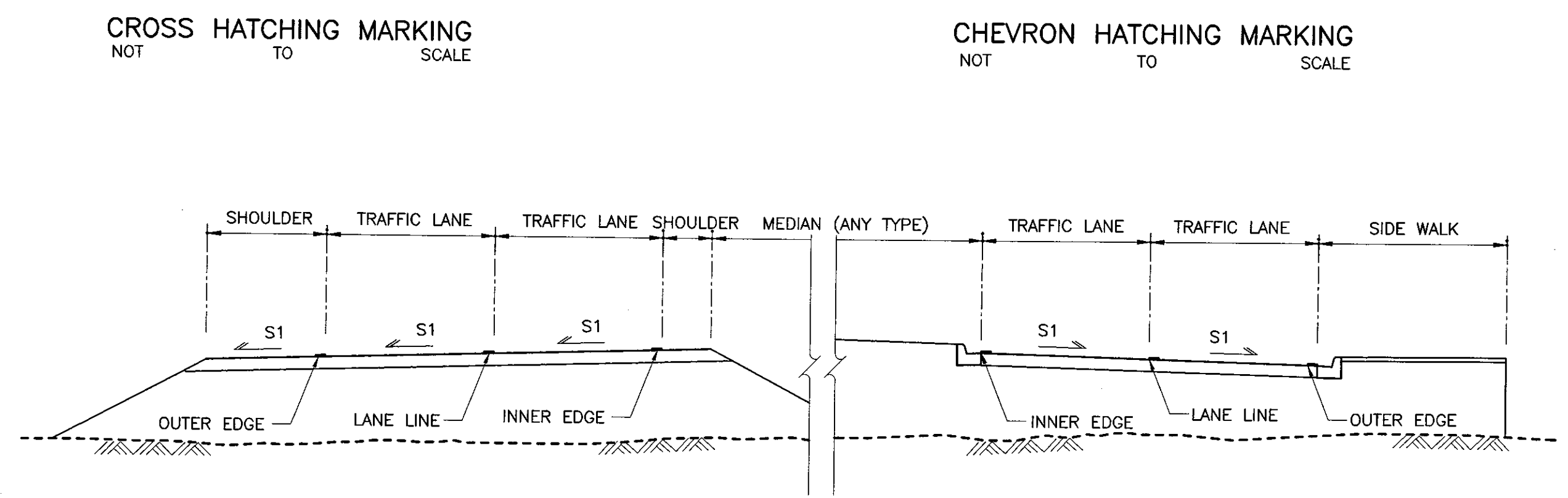
MARKING AT PAVEMENT NOT TO SCALE
